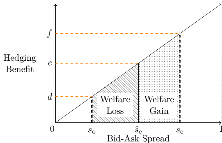
Figure 7 – Cheap Substitution
