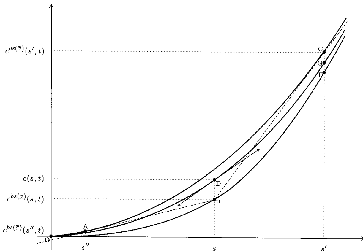
Figure 3. Bounds on a call's price and delta. The curve OAC (respectively, OBF ) is the Black-Scholes call price computed as a function of the underlying price using the upper bound, \bar{\sigma}(t) (lower bound, \underline{\sigma}(t) ), on the true volatility. The two curves bound the true call price curve ODG . The true hedge ratio given a stock price of s is bounded from above by the slope of BC and from below by the slope of AB ; both tangents from B to OAC . c(s, t) is the time t value of a call option written on a asset worth s . c^{bs(\bar{\sigma})}(s, t) is the time t Black-Scholes value of a call option written on an asset worth s when the asset's volatility is the deterministic function \bar{\sigma}(t) . c^{bs(\underline{\sigma})}(s, t) is similarly defined.
