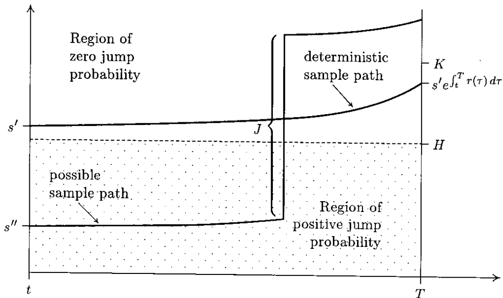
Figure 4a. Two sample paths of a non-proportional mixed diffusion-jump process for which the ‘no-crossing’ property is violated. The path that starts out lower has a positive probability of finishing above K at time T . The path that starts out higher always finishes below K . A call option with exercise price K and time T maturity will be such that c(s', t) = 0 , yet c(s'', t) > 0 .
