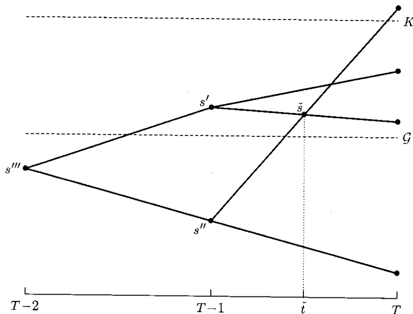
Figure 4b. A non-recombining binomial tree for which the ‘no-crossing’ property is violated. If the process reaches s' , it will always finish below K and a call with an exercise price of K and a time T maturity will be valueless. But if the process reaches s'' , the process can finish above K and the call has a positive price.
