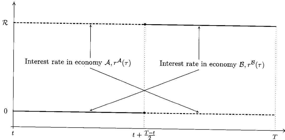
Figure 2a. Interest rate time profiles in two otherwise equivalent economies \mathcal{A} and \mathcal{B} . One profile is a time permutation of the other with \int_t^T r^{\mathcal{A}}(\tau) d\tau = \frac{T-t}{2} \mathcal{R} = \int_t^T r^{\mathcal{B}}(\tau) d\tau . Therefore riskless bonds that promise the same payoff at time T have the same price in both economies.
