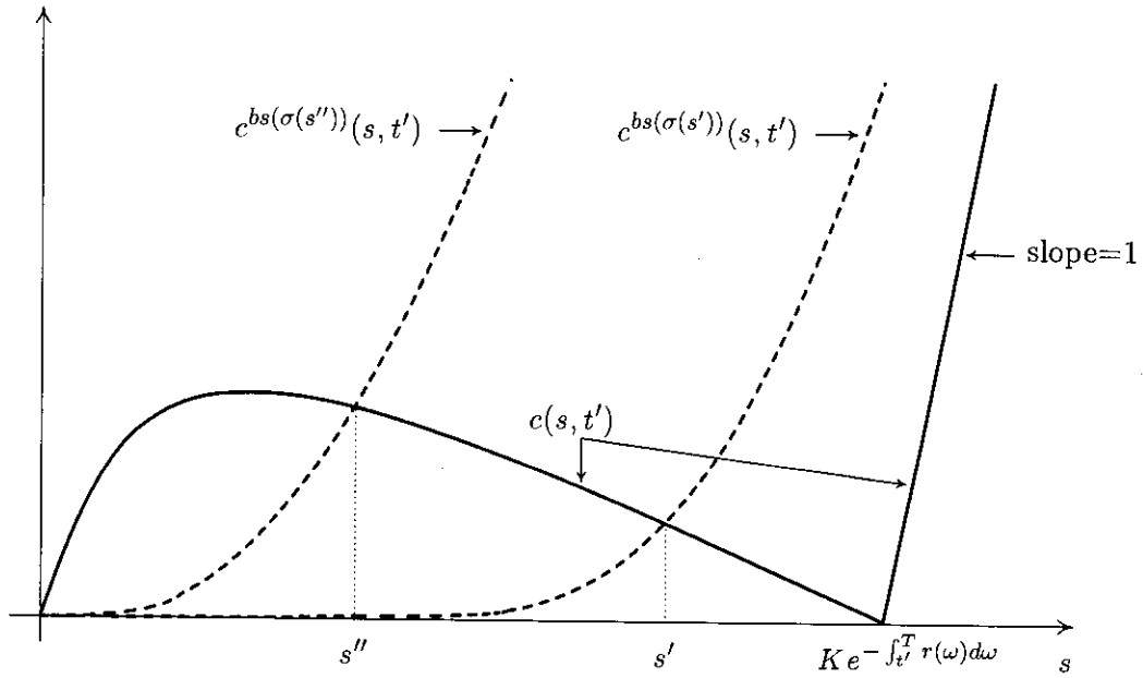
Figure 5a. The relation between c(s, t') and s in a non-Markovian setting. The call price function is non-monotonic and non-convex. c(s, t') is the time t' value of a call option written on an asset worth s . c^{bs}(\sigma(s'))(s, t') is the time t' Black-Scholes value of a call option written on an asset worth s when the asset's volatility is constant and equal to \sigma(s') . c^{bs}(\sigma(s''))(s, t') is similarly defined.
