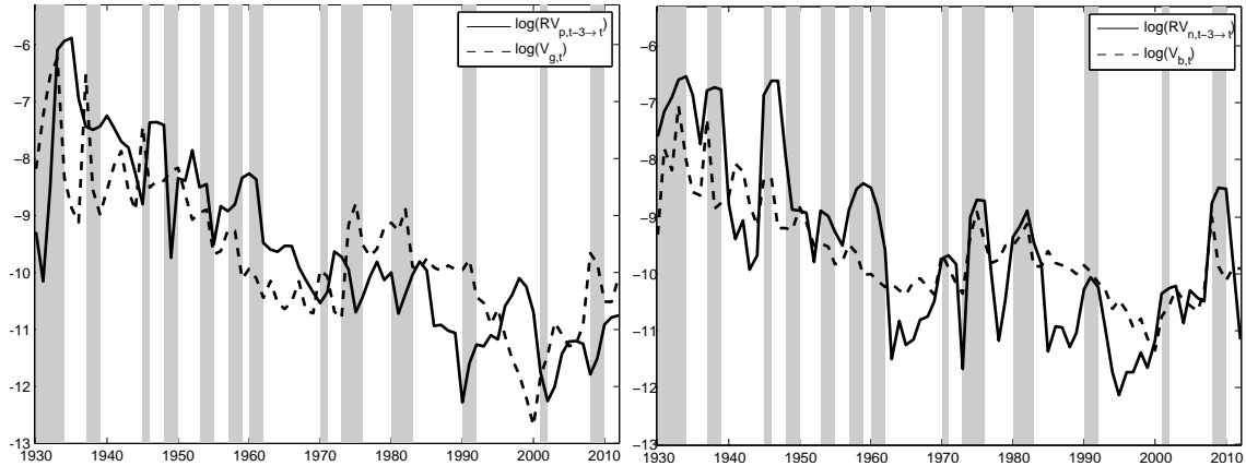
Figure 3: Realized and Predictive Log Volatilities
