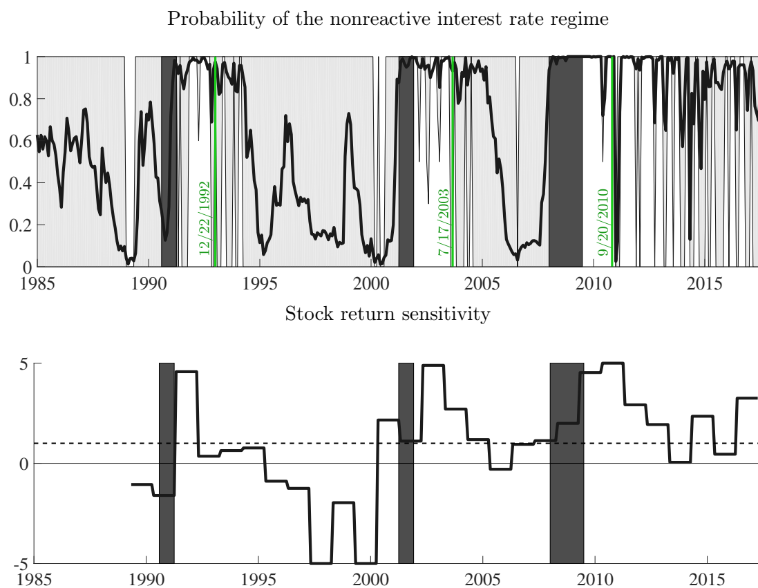
Figure 10: Regime probability
