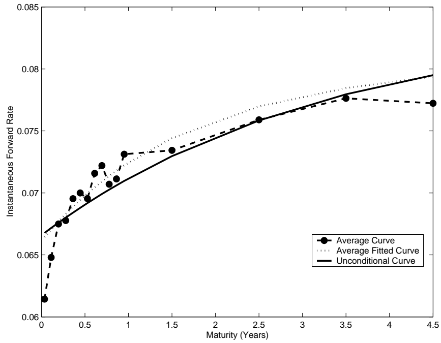
Figure 3: Unconditional Curve, “Average” Curve and average fitted curve of CFRS Model, Fama-Bliss Treasury Data, June 1964 to March 2000
